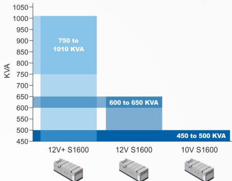
Diesel Generator Range for Series 1600 Engine
